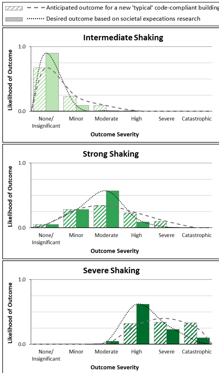
Figure I3. Distribution of anticipated and desired outcomes for a new 'typical' Code-complaint building in terms of related to Protection of Property.
