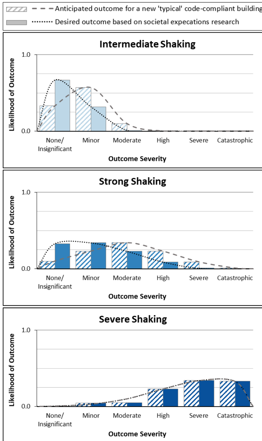
Figure I5. Distribution of anticipated and desired outcomes for a new 'typical' Code-complaint building in terms of related to Protection of Amenity & Function.
