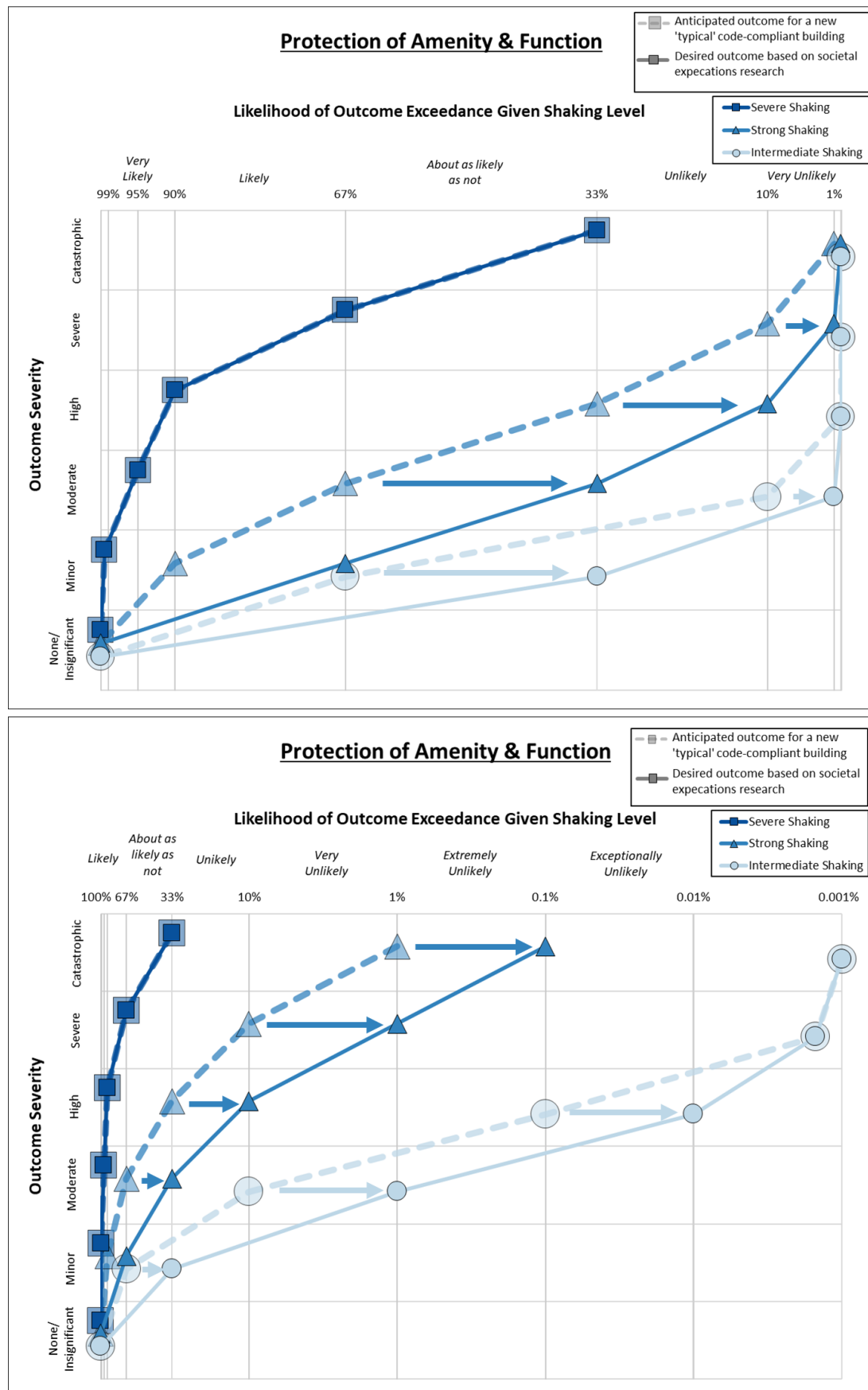
Figure I6. Cumulative distribution of anticipated and desired outcomes a new 'typical' Code-complaint building in terms of Protection of Amenity & Function (linear scale top and logarithmic scale bottom).
