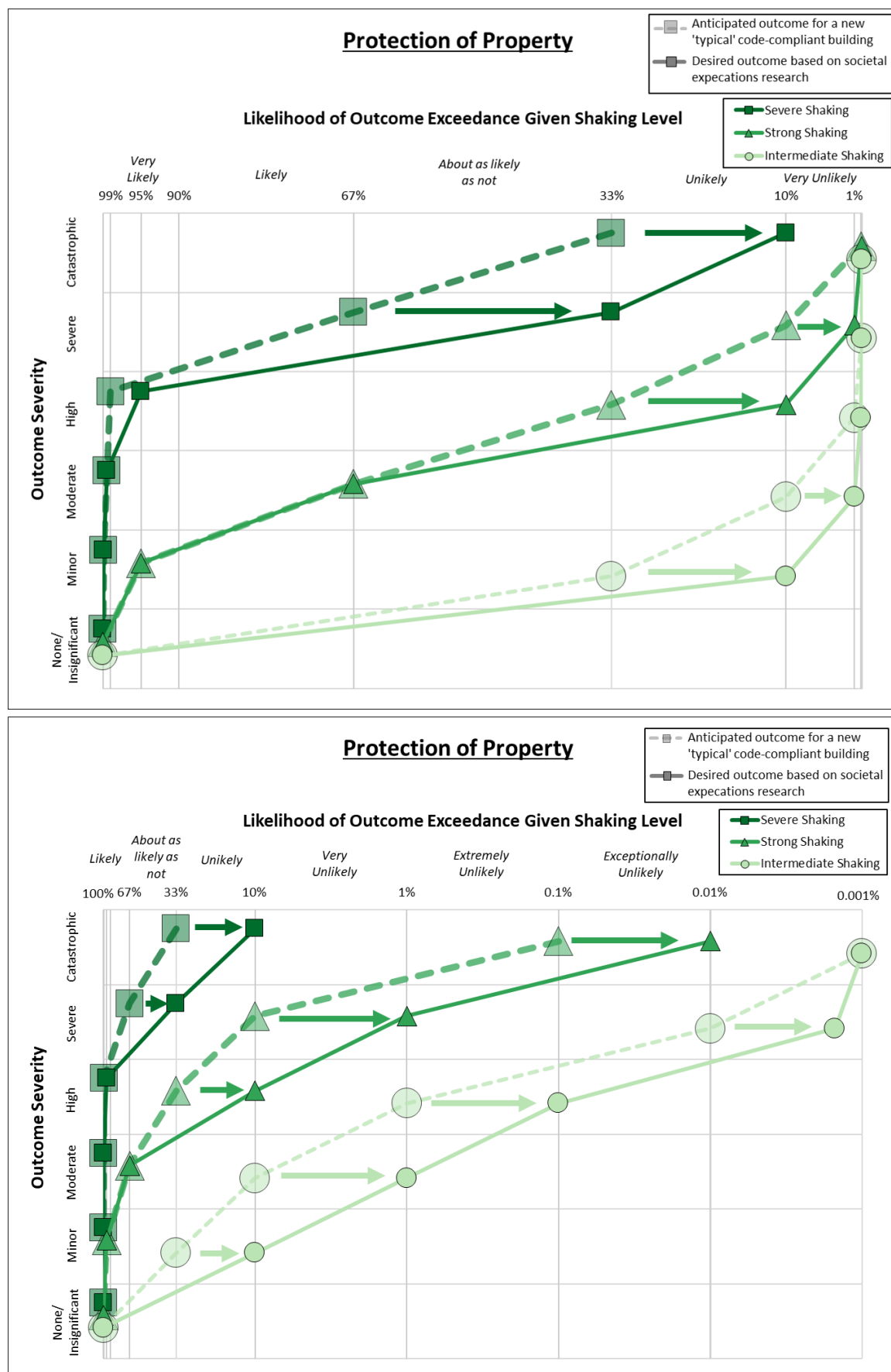
Figure 14. Cumulative distribution of anticipated and desired outcomes for a new 'typical' Code-complaint building in terms of Protection of Property (linear scale top and logarithmic scale bottom).
