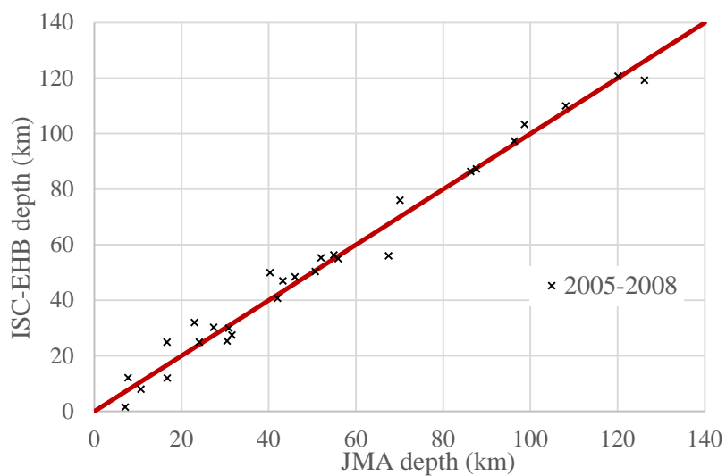
Figure 1.8 Depth correlation between JMA and ISC-EHB catalogues for earthquakes between 2005 and 2008 with strong-motion records that will be used for developing GMPEs for Japan.
