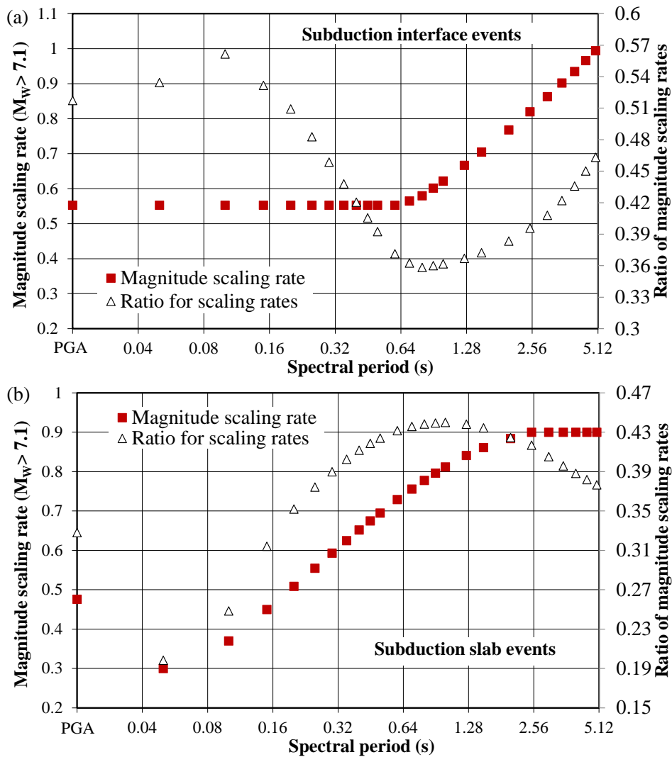
Figure 3.11 Magnitude scaling coefficient d_{int} for large subduction interface events and the ratio d_{int}/c_{int} events in (a) and d_{SL} for large subduction slab events and the ratio d_{SL}/c_{SL} in (b).
