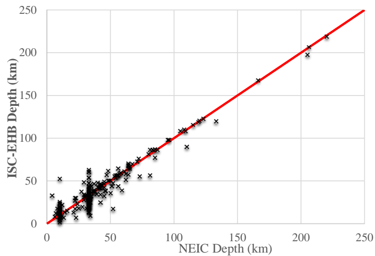
Figure 1.4 Depth correlation between NEIC and ISC-EHB catalogues for those events between 1996 and 2008 with strong-motion records suitable for developing GMPEs.
