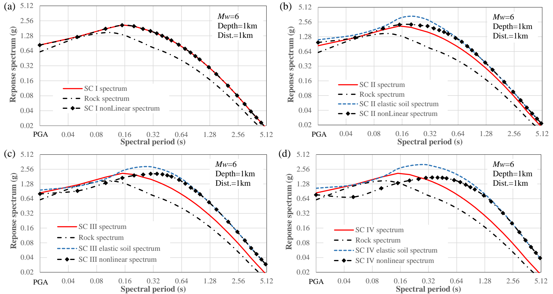
Figure 3.52 Predicted response spectra for an M_w=6 shallow crustal event with a fault-top depth of 1km, a reverse or strike-slip faulting mechanism, and at a distance of 1km for SC I sites in (a), SC II site in (b), SC III sites in (c) and SC IV sites in (d), together with rock spectrum, elastic soil spectrum and nonlinear soil spectrum.
