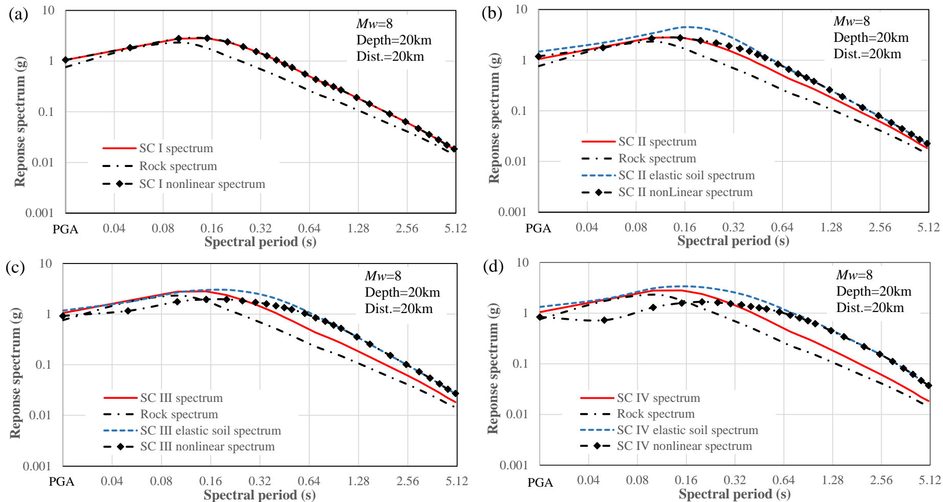
Figure 3.59 Predicted response spectra for an M_w=8 shallow interface event with a fault-top depth of 20km, and at a distance of 20km for SC I sites in (a), SC II site in (b), SC III sites in (c) and SC IV sites in (d), together with rock spectrum, elastic soil spectrum and nonlinear soil spectrum.
