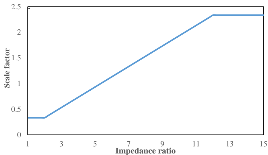
Figure 2.6 Scale factor accounting for site impedance ratio.
