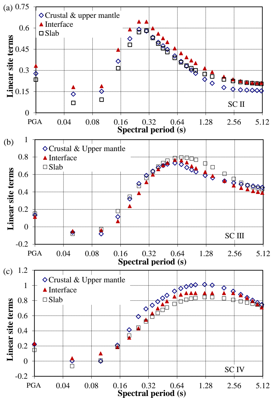
Figure 3.44 Comparison of linear-site terms for (a) SC II sites, (b) SC III sites and (c) SC IV sites from the models for shallow crustal and upper mantle earthquakes, subduction interface events and subduction slab events.
