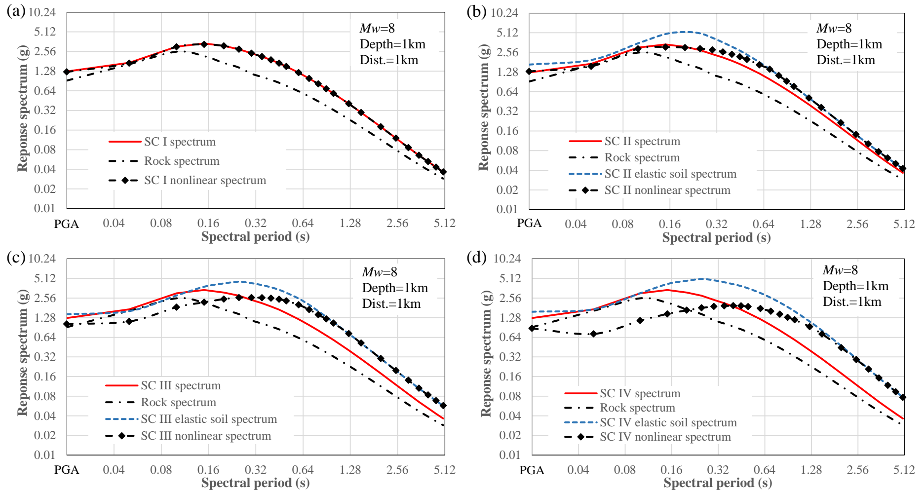
Figure 3.54 Predicted response spectra for an M_w=8 shallow crustal event with a fault-top depth of 1km, a reverse or strike-slip faulting mechanism, and at a distance of 1km for SC I sites in (a), SC II site in (b), SC III sites in (c) and SC IV sites in (d), together with rock spectrum, elastic soil spectrum and nonlinear soil spectrum.
