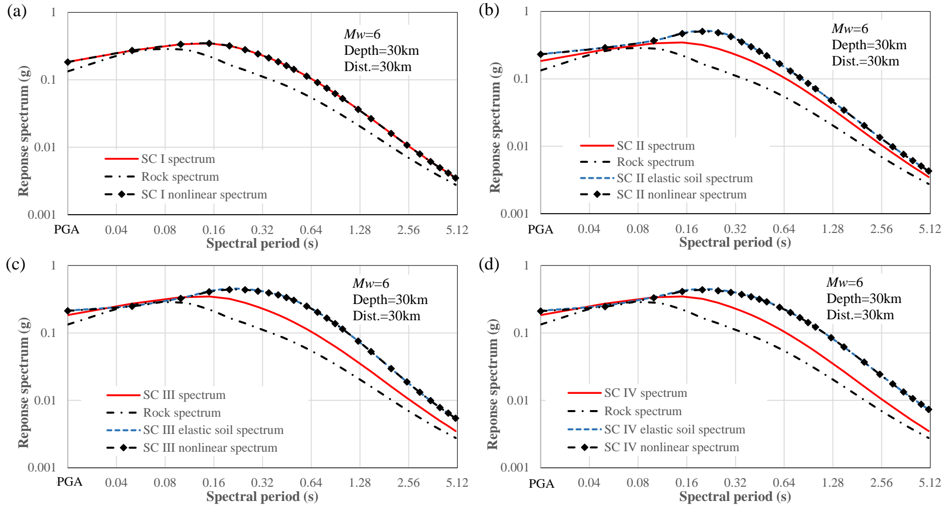
Figure 3.65 Predicted response spectra for an M_w=6 slab event with a fault-top depth of 30km, and at a distance of 30km for SC I sites in (a), SC II site in (b), SC III sites in (c) and SC IV sites in (d), together with rock spectrum, elastic soil spectrum and nonlinear soil spectrum.
