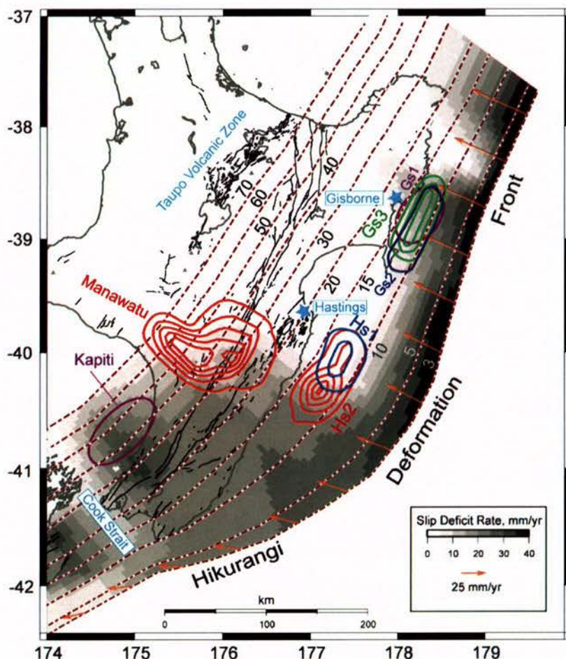
Figure 3 Estimated slip distributions of major NZ slow-slip events through November 2007; two other events (not shown) started in December 2007. Slab contours (in km, dashed lines), interplate coupling distribution (shown as slip rate deficit), convergence vectors (red arrows) and locations of slow-slip events (coloured contours). Locking distribution is updated from Wallace et al. (2004). Slow-slip events are shown as 50 mm contours of slip on the plate interface, and as ellipses when only the general location is known (Gs1 and Kapiti). The times of the events are given below.
