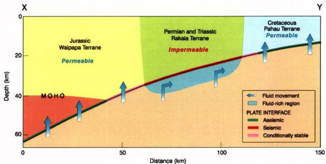
Figure 4. A conceptual model of fluid movement and the nature of plate coupling beneath the southern North Island, along the depth section shown in Fig. 3.
