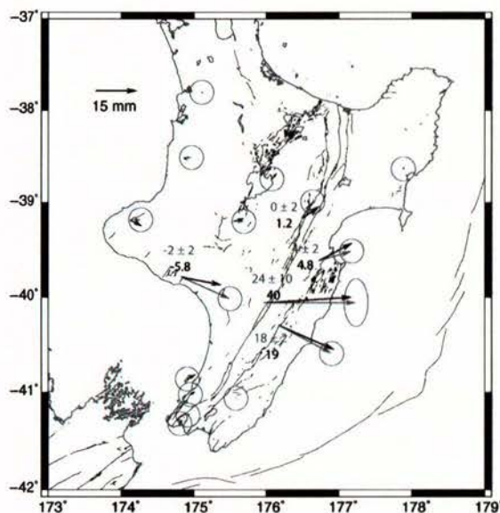
Fig. 10 Fit between observed (grey arrows) and calculated (black arrows) horizontal offsets over the whole duration of the Manawatu event. The numbers beside each site show the observed (grey) and calculated (black) vertical offsets in mm.
