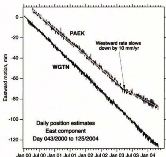
Fig. 6 Eastward motion of sites PAEK and WGTN (Figure 1) relative to the Australian Plate. PAEK slowed by \sim 10 mm/yr in about April 2003. At the same time its vertical (upward) rate increased by \sim 10 mm/yr. Soon after the end of this plot, the velocities returned to approximately their earlier values.
