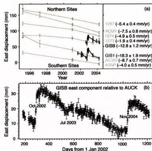
Fig. 4 (a) Position time series relative to a site near Auckland for campaign GPS sites north and south of Gisborne, and for selected days of CGPS sites GISB and GIS1 (Figure 1). The campaigns are too infrequent to detect the events seen at the CGPS sites. (b) GISB time series showing eastward surface displacements of 20-25 mm occurring over 7-10 day periods in 2002 and 2004, with a smaller and slower event in 2003.
