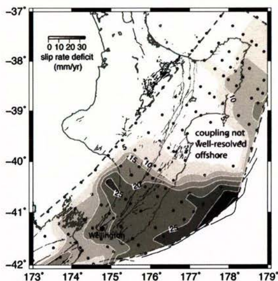
Fig. 3 Distribution of seismic coupling on the Hikurangi subduction interface, estimated from ~12 years of campaign GPS site velocities using an elastic crustal block model. The dots are the nodes at which slip deficit is estimated, with bilinear interpolation between nodes. Darkest areas represent slip deficit of 30 mm/yr, meaning this amount of slip is being stored as elastic energy for eventual release as slip on the subduction interface, probably in a large earthquake. White areas imply slip is occurring steadily with no elastic strain build up. The coupling distribution offshore of the eastern North Island is not well resolved. There is also strong coupling, not shown in the figure, on the strike-slip faults in the northern South Island and southern North Island.
