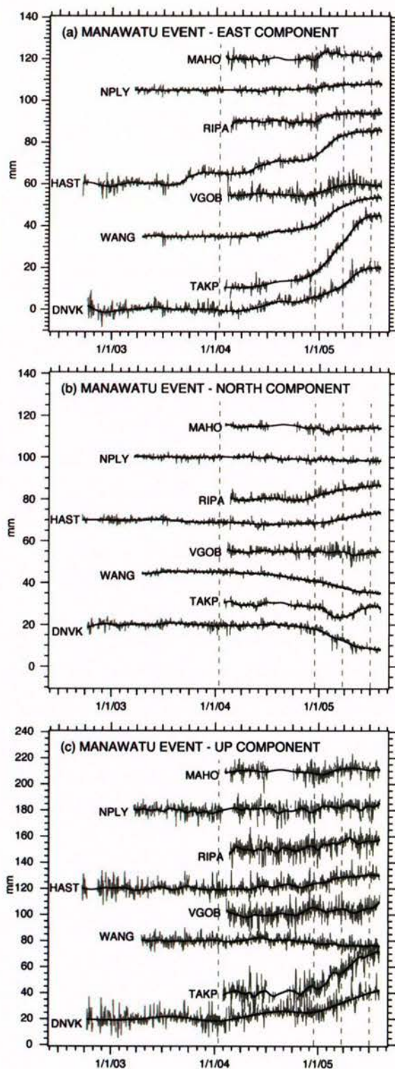
Fig. 8 Daily and smoothed time series from CGPS sites (Figure 1) affected by the Manawatu slow-slip event. The grey dashed lines split the event into three sub-events that we model separately.
