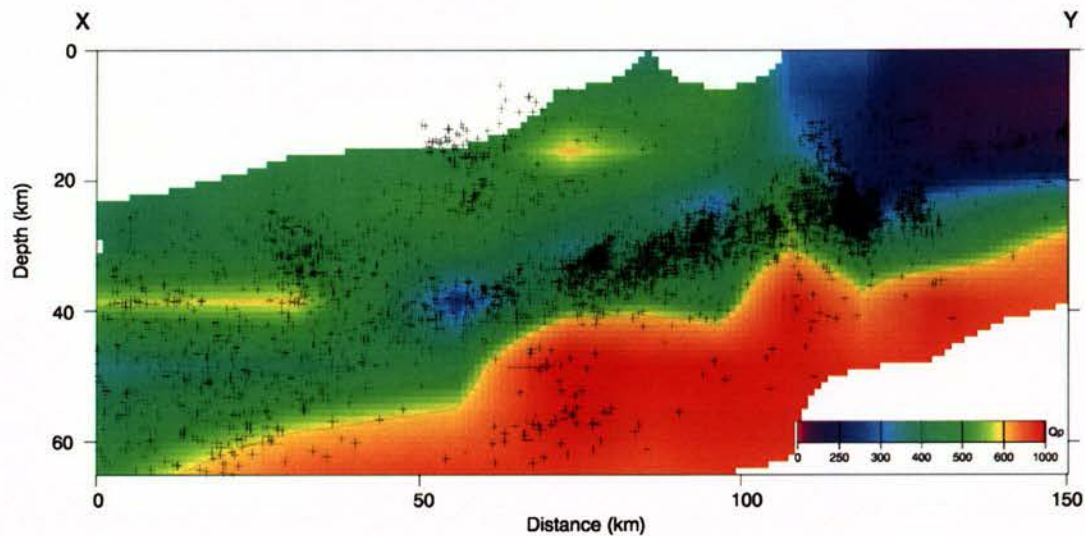
Figure 3. Down-dip depth section through the region of strong plate coupling (see Fig. 1 for location). Relocated earthquakes within 10 km of the section are shown, together with the distribution of Q_p [Eberhart-Phillips et al. , 2005].
