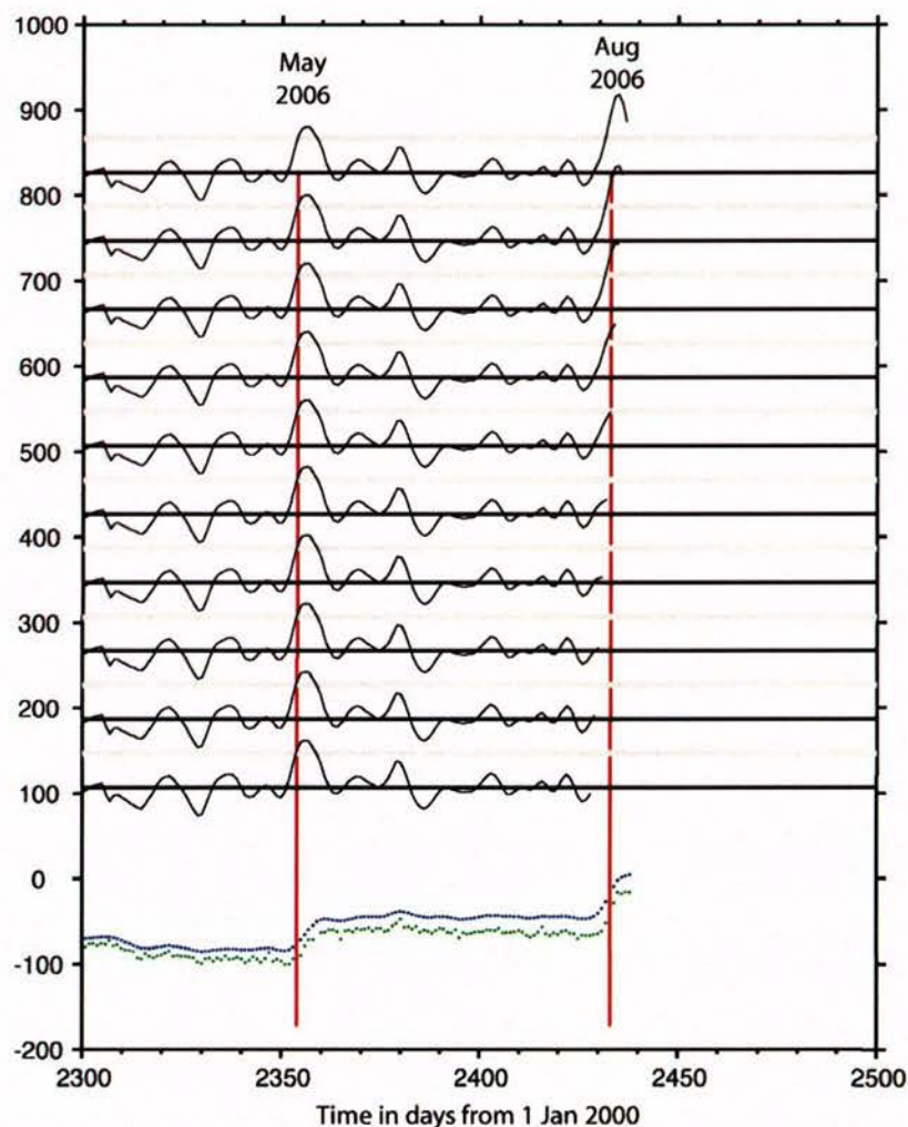
Figure 5 Cross-correlation functions (CCF) for two slip events offshore of Hastings (May and August 2006) using the 3-day ramp function. The time series at bottom is the east component of site PAWA (blue is low-pass filtered, green is unfiltered). The black curves are the CCF calculated using all available GPS data (not just PAWA) for time periods ending at days 2436 (bottom curve) through 2445 (top curve). In each case, the gray horizontal bar is 1 unit above zero (black horizontal line). The vertical red lines show the day at which the CCF reaches a value of 1, our initial detection threshold. For the first event, the detection threshold is reached about 3 days into the event; for the second it is about 4 days.
