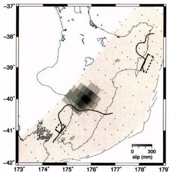
Fig. 9 Slip distribution on the subduction interface over the total duration of the 2004-05 Manawatu slow-slip event. Black lines show the transition from relatively strong to relatively weak coupling in the southern North Island and Gisborne regions, from Figure 3. Black rectangles (solid where well constrained, dashed otherwise) show inferred locations of slow-slip in the Gisborne and Kapiti events. All events lie near or below the coupling transition.
