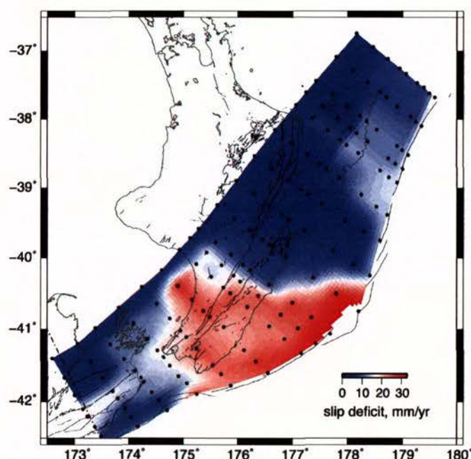
Figure 2 Distribution of interplate coupling on the Hikurangi subduction interface, estimated from ~12 years of campaign GPS site velocities using an interacting elastic crustal block model. The dots are the nodes at which slip deficit is estimated, with bilinear interpolation between nodes. Red areas show a slip deficit of 30 mm/yr, meaning this amount of slip is being stored as elastic energy for eventual release as slip on the subduction interface, probably in a large earthquake. Dark blue implies slip is occurring steadily with no elastic strain build up. The coupling distribution offshore of the eastern North Island is not well resolved. There is strong coupling on the strike-slip faults in the northern South Island and southern North Island, but this is not shown on this figure.
