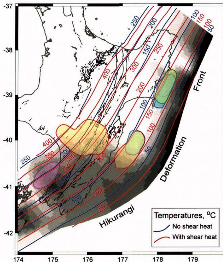
Figure 6 Estimates of temperature (red and blue contours) on the Hikurangi thrust interface and the general locations of slow-slip events (coloured regions). The gray areas are the locking distribution from Wallace et al. (2004). Temperatures were estimated by taking into account the age and rate of the incoming subducting lithosphere and the geometry of the margin. Blue temperature contours do not include shear heating while red contours include heating from 20 MPa of shear stress on the plate interface. In either case, the slow-slip events off the coast of the north and central North Island occur at temperatures lower than about 150°C.
