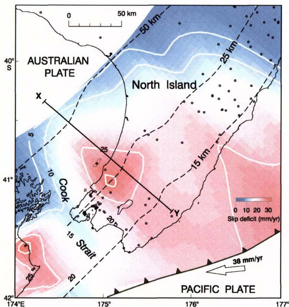
Figure 1. Tectonic setting of the southern North Island of New Zealand. Coloured contours show the slip rate deficit distribution at the plate interface (updated from Wallace et al. [2004] ), and dashed lines show isobaths of the plate interface determined from earthquakes relocated in this study. X-Y is the location of the depth section shown in Fig. 3.
