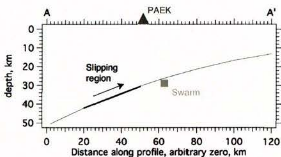
Fig. 7 Cross-section from northwest (A) to southeast (A') showing inferred region of slow-slip, PAEK CGPS station, and the site of several earthquake swarms located near the top of the subducting plate. Coulomb stress changes calculated from the slip event favour the normal faulting style of the swarm earthquakes.
