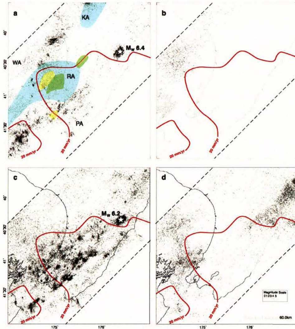
Figure 2. Relocated seismicity for the period 1990-2005. In all plots, dashed lines show the limit of the earthquake sample and red lines are the 20 mm/yr slip rate deficit contours on the plate interface determined from GPS (see Fig. 1). Stars show the two largest earthquake sequences during the study period. a) Earthquakes in the overlying plate crust (depth < 40 km). Legend for geological terranes: KA – Kaweka; PA – Pahau; RA – Rakaia; WA – Waipapa. Coloured regions show seismological evidence for strong terranes in the mid crust: blue – group velocity > 2.9 km/s for 13s Rayleigh waves (sampling range \sim 10 -15 km; Lin et al. [2007] ); yellow – V_p > 6.5 km/s and green – Q_p > 500 (both at 15 km depth; Eberhart-Phillips et al. [2005] ). b) Earthquakes in the mantle nose of the overlying plate (depth \geq 40 km). c) Earthquakes in the upper plane of the dipping seismic zone (i.e. within 15 km of the plate interface). d) Earthquakes in the lower plane of the dipping seismic zone.
