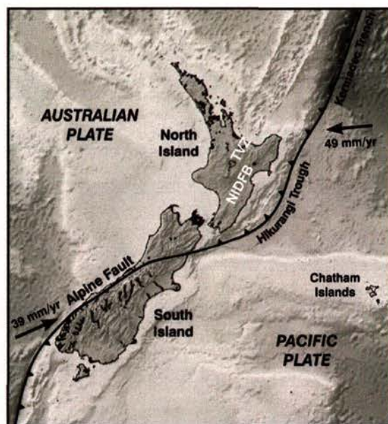
Fig. 2 Tectonic setting of New Zealand. Light coloured areas are submerged continental crust. Pacific Plate subducts beneath North Island at the Hikurangi Trough. TVZ: Taupo Volcanic Zone; NIDFB: North Island Dextral Fault Belt.
