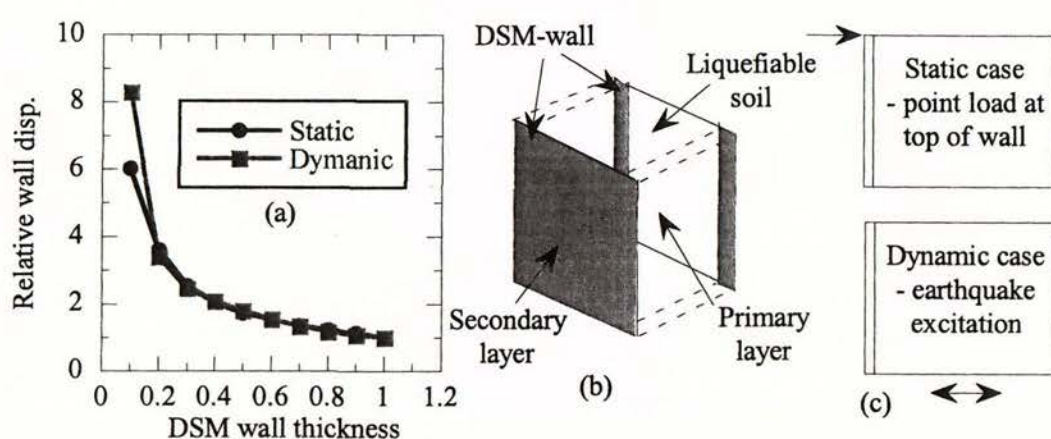
Figure 5.4 Relative displacement of wall as a function of DSM-wall thickness
