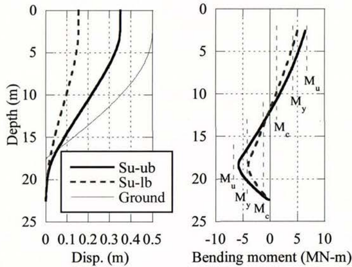
Figure 3.15 Pile response for a lateral spreading case with U_{G2} = 0.5\text{m} and \beta = 1/50 , showing the effects of changing the ultimate pressure in the liquefied soil
