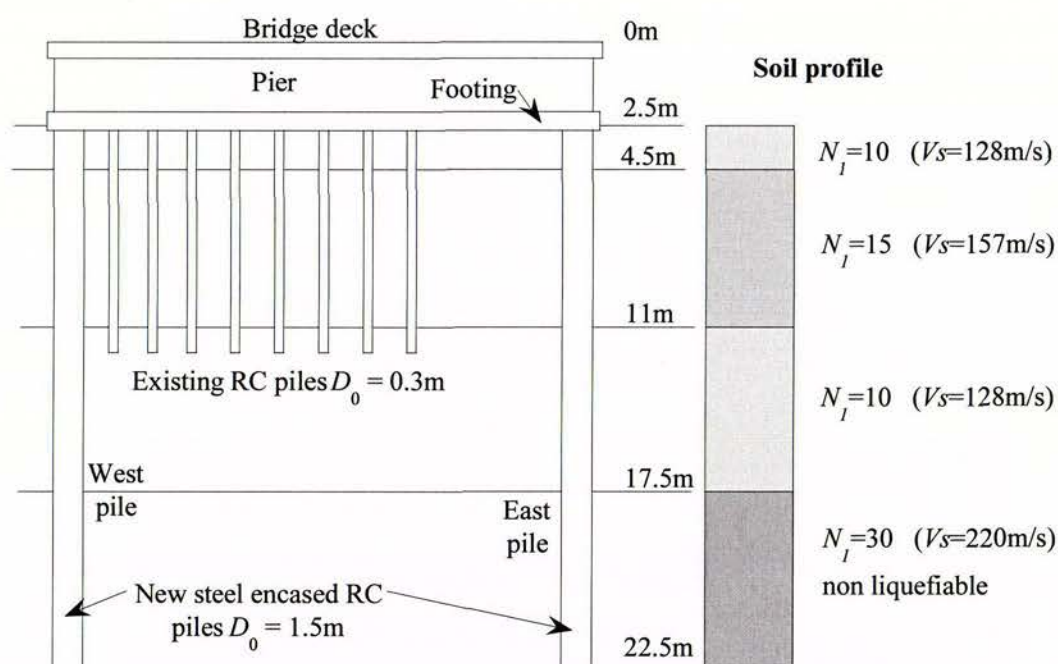
Figure 4.4 Central pier of bridge: (a) Foundation layout, (b) soil properties used in analysis
