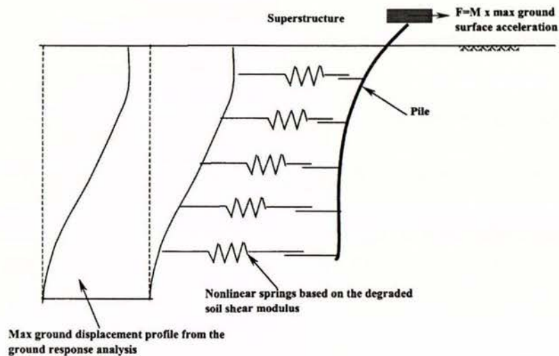
Figure 2.30 Beam on spring foundation model for pseudo-static analysis (Liyanaathirana and Poulos 2005)
