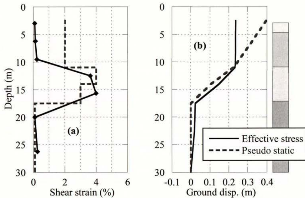
Figure 4.22 Comparison between the free field ground response calculated from the effective stress and psuedo static methods; (a) maximum cyclic shear strain, (b) ground displacement
