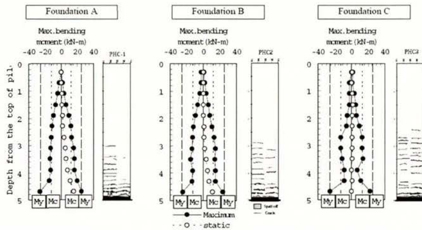
Figure 2.16 Measured maximum moments and observed crack patterns for piles during the lateral spreading experiment (Yasuda et al. 2000). Foundation A experienced the most lateral ground displacement and Foundation C experienced the least.
