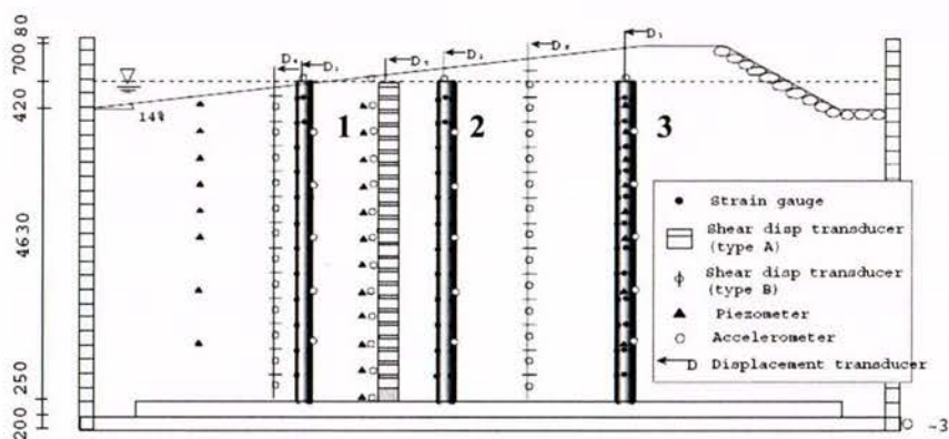
Figure 2.15 Full scale lateral spreading experiment on piles (Yasuda et al. 2000)
