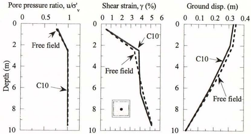
Figure 5.8 Computed response of soil inside the C-10 DSM-wall using a single layer mesh (conventional 2D model)
