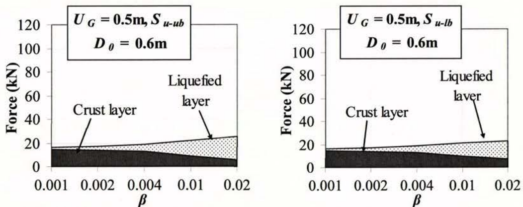
Figure 3.18 Force applied to flexible piles from the crust and liquefied layers as a function of the stiffness degradation due to liquefaction, \beta
