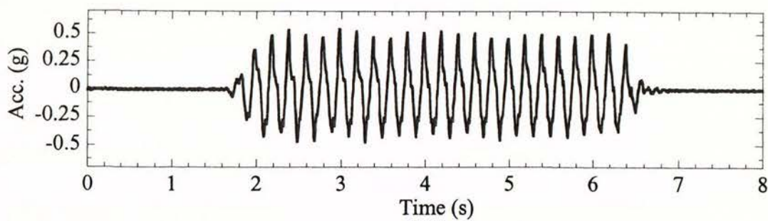
Figure 5.18 Horizontal accelerations recorded at the shake table
