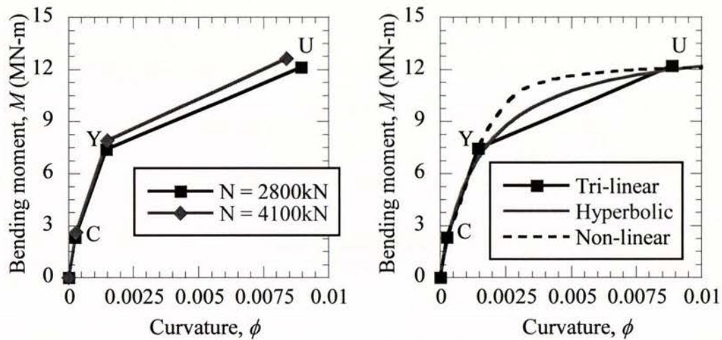
Figure 4.5 Moment curvature relationships for D_0 = 1.5m pile: (a) effect of axial load on M-\phi curve, (b) fitting hyperbolic curve to tri-linear relationship
