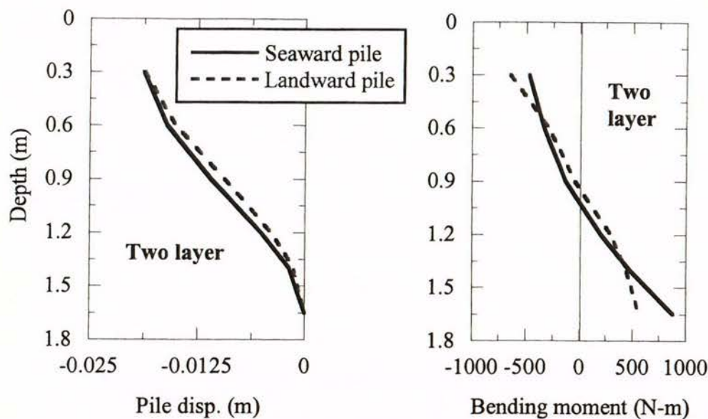
Figure 5.27 Pile response for the elongated model using a double layer analysis; (a) peak lateral pile displacement, (b) peak pile bending moment
