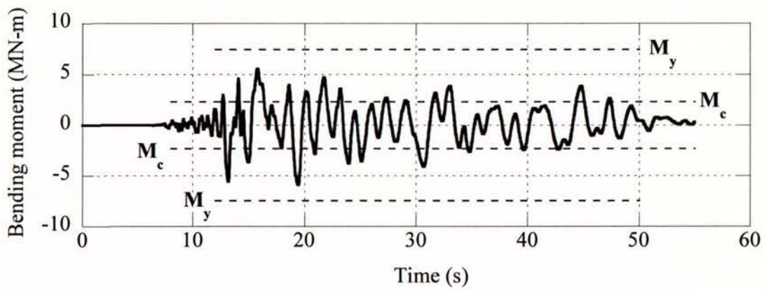
Figure 4.20 Bending moment time history at the pile head calculated using the non-linear base layer model
