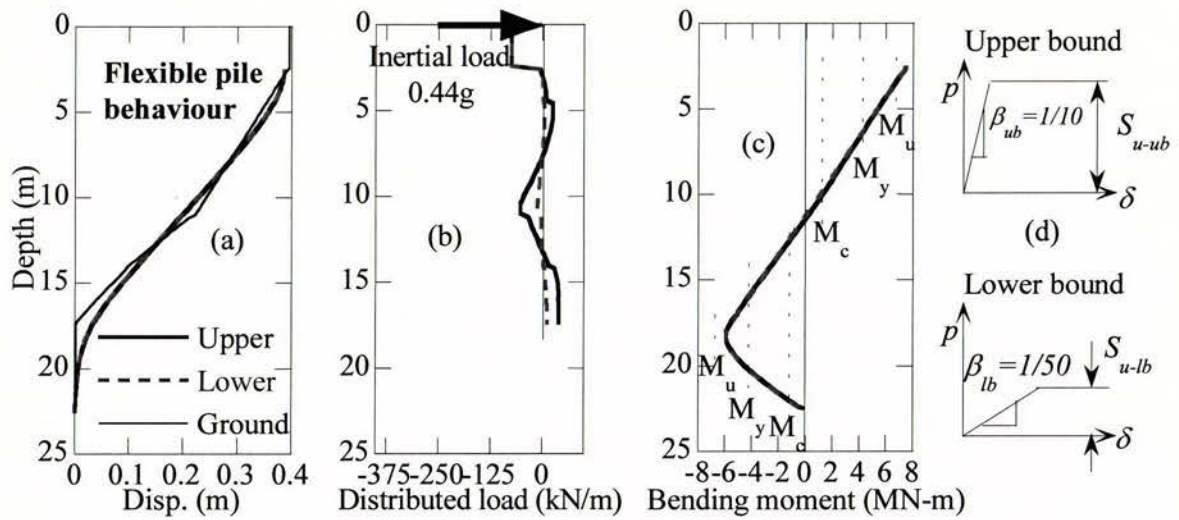
Figure 3.13 Variation of pile response due to liquefied layer properties for a cyclic phase case with a large inertial load, showing pile displacement, distributed load on the pile and pile bending moment
