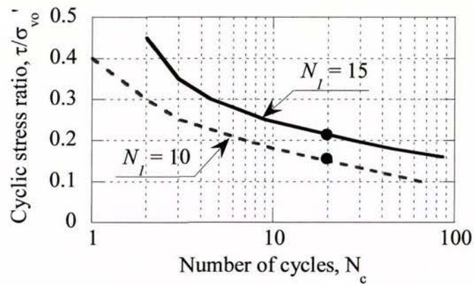
Figure 4.7 Simulated liquefaction resistance curves for N_1=10 and N_1=15 soil layers
