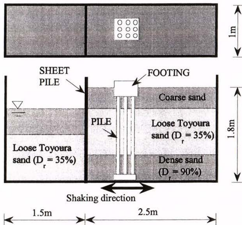
Figure 5.17 Schematic plot and plan and side view of the soil pile model used in the experiment (after Cubrinovski et al. 2005)
