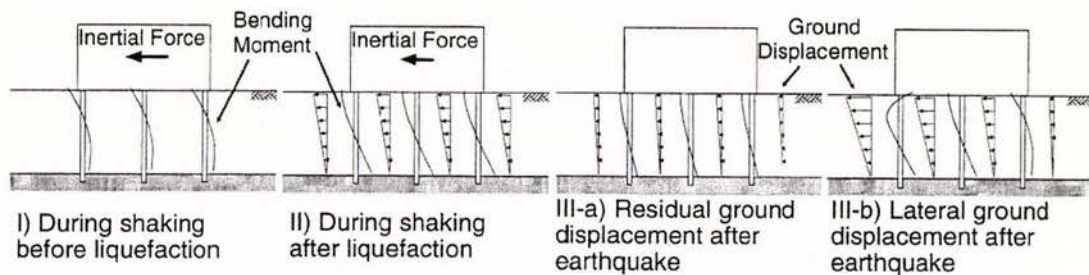
Figure 2.1 Schematic figure showing soil-pile interaction in liquefiable soils (Tokimatsu and Asaka 1998). The inertial force and ground displacement acting on piles at different stages of the loading are shown, with the resulting pile bending moments.
