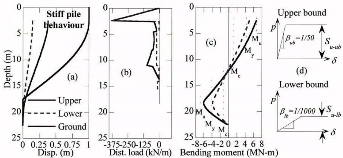
Figure 3.14 Variation of pile response due to liquefied layer properties for a lateral spreading case with U_{G2} = 1m , showing pile displacement, distributed load on the pile and pile bending moment
